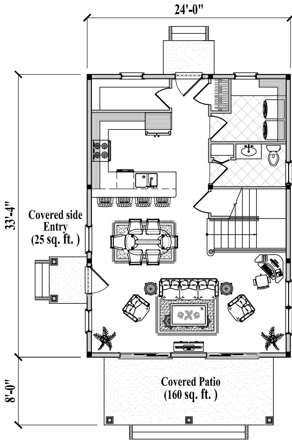
Lower Floor Plan (800 sq. ft. or 74.3 m 2 )
