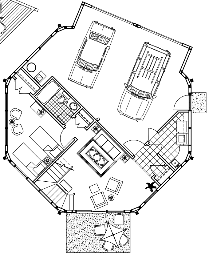
Lower Floor Plan (1,195 sq. ft.)
