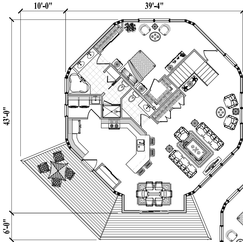
Upper Floor Plan (1,330 sq. ft. or 123.5 m 2 )
