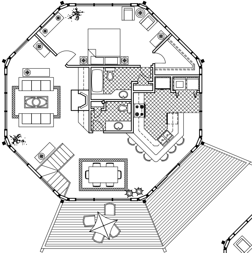
Upper Floor Plan (1,125 sq. ft.)
