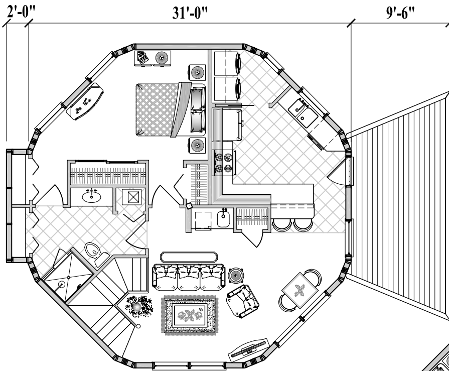
Upper Floor Plan (820 sq. ft. or 76.2 m 2 )
