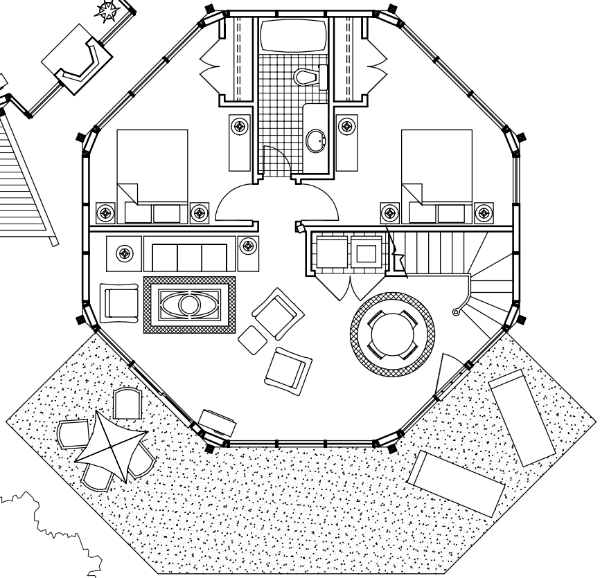
Lower Floor Plan (800 sq. ft.)
