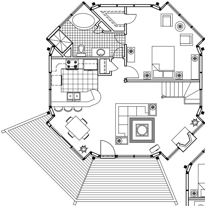
Upper Floor Plan (900 sq. ft.)
