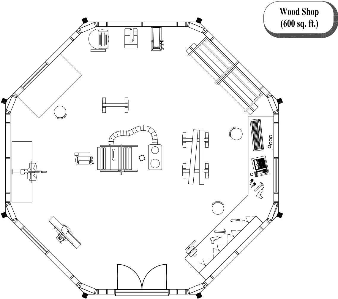
Floor Plan (600 sq. ft.)
