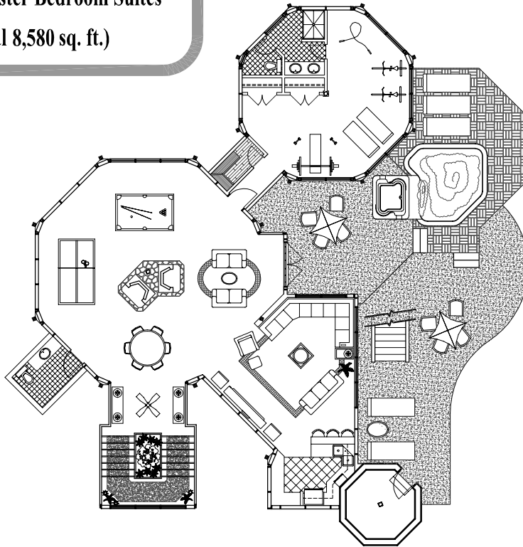
Lower Level Floor Plan (2,250 sq. ft.)
