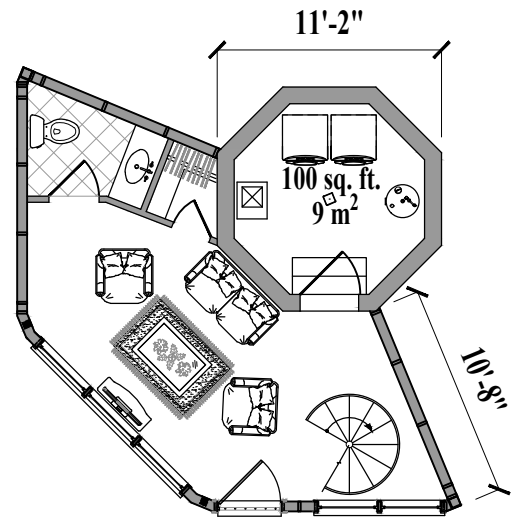
Lower Floor Plan (Total 390 sq. ft. or 35 m 2 including Pedestal)
