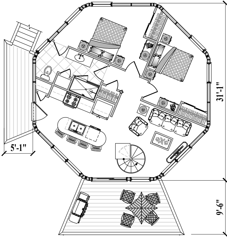
Floor Plan ( Total 800 sq. ft. or 75m 2 )
