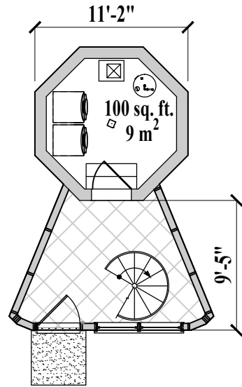
Lower Floor Plan ( Total 215 sq. ft. or 20 m 2 including Pedestal )
