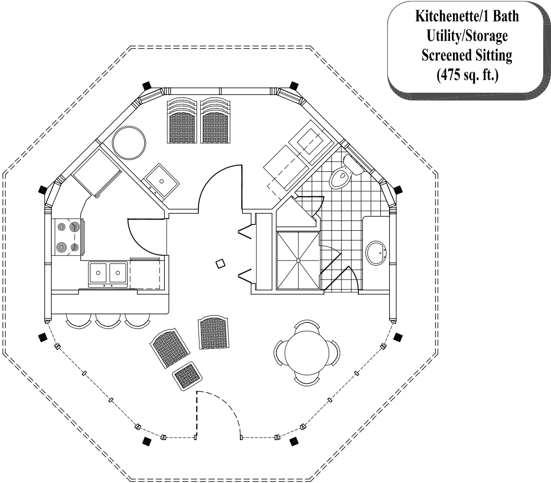
Floor Plan (475 sq. ft.)
