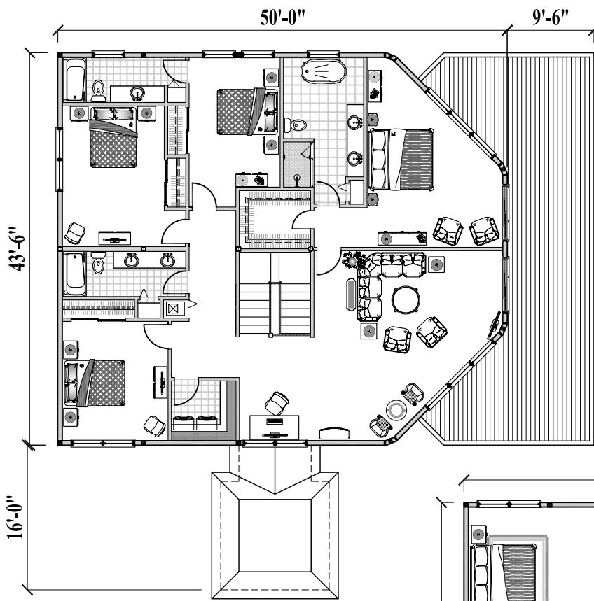
Upper Floor Plan (2,000 sq. ft. or 186 m 2 )
