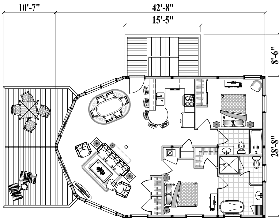
Upper Floor Plan (1,115 sq. ft. or 103.5 m 2 )
