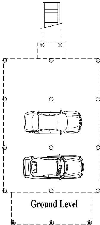
Lower Floor Plan (800 sq. ft. or 74.3 m 2 )
