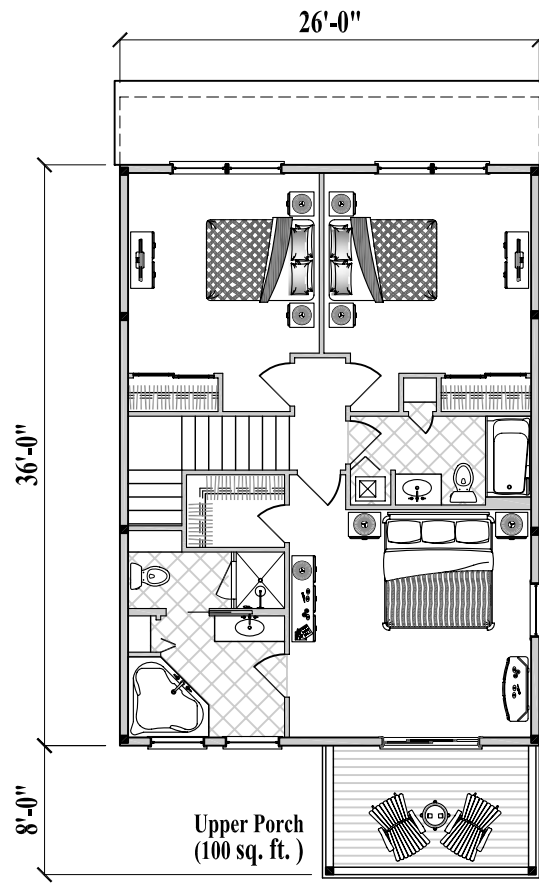
Upper Floor Plan (940 sq. ft. or 87.3 m 2 )
