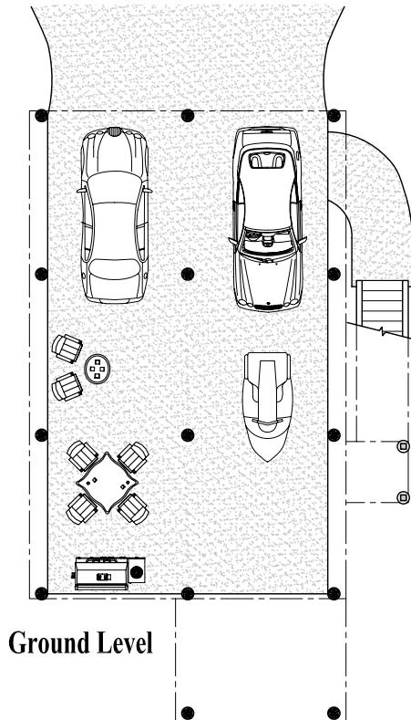
Lower Floor Plan (1,040 sq. ft. or 96.6 m 2 )
