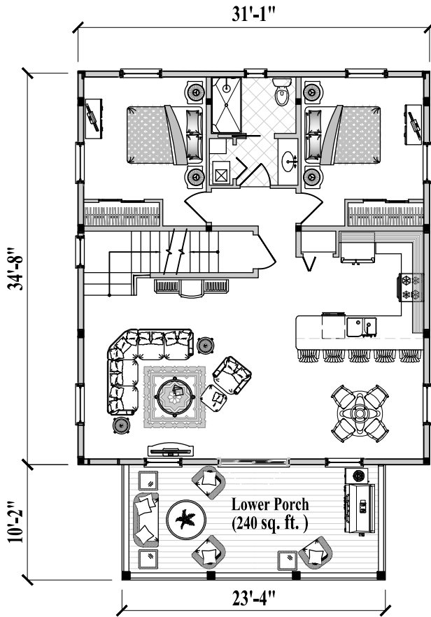
Lower Floor Plan (1,085 sq. ft. or 100.7 m 2 )
