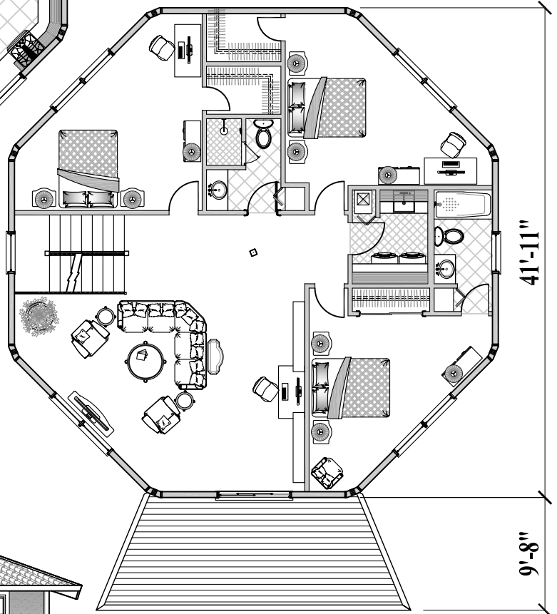
Lower Floor Plan (1,450 sq. ft. or 135 m 2 )
