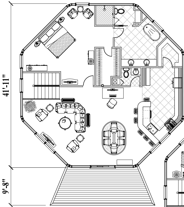
Upper Floor Plan (1,450 sq. ft. or 135 m 2 )
