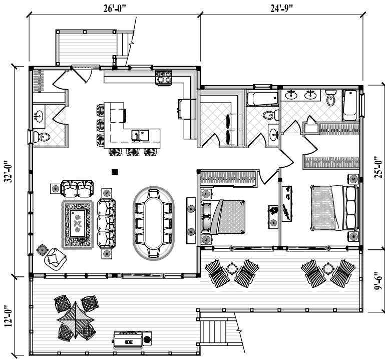
Floor Plan (1,450 sq. ft. or 135 m 2 )
