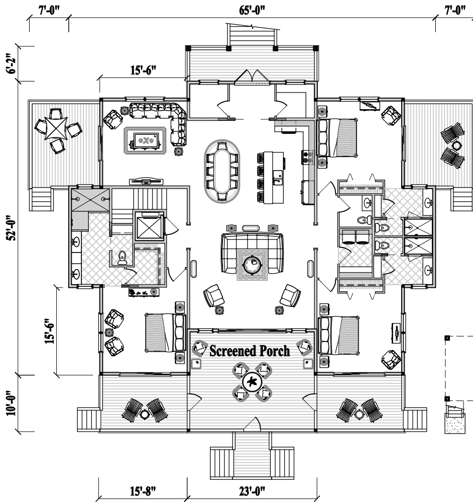
Floor Plan (2,745 sq. ft. or 255 m 2 )
