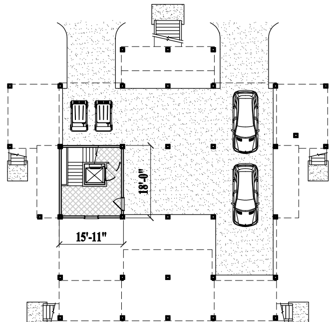
Ground Level (Parking Area) (285 sq. ft. or 26.5 m 2 )
