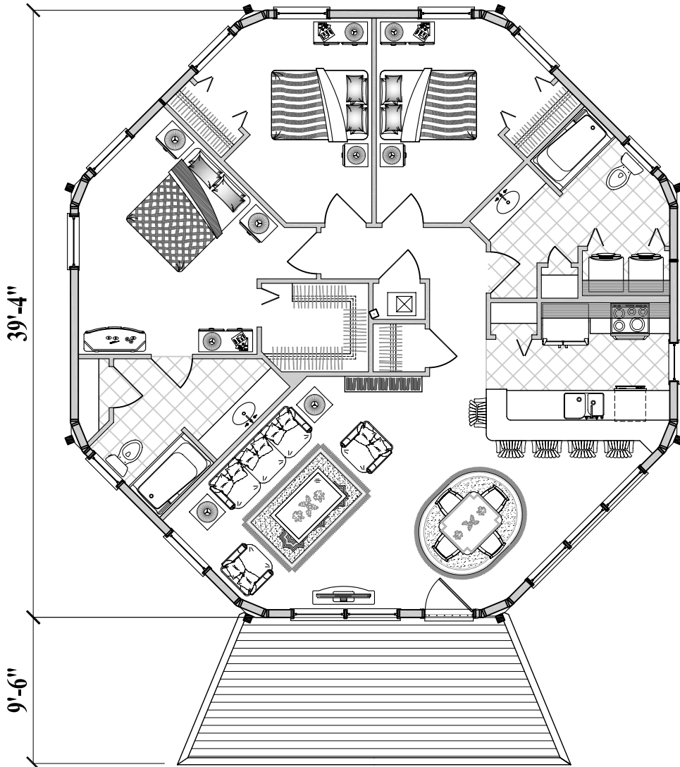
Floor Plan ( Total 1,280 sq. ft. or 119 m 2 )
