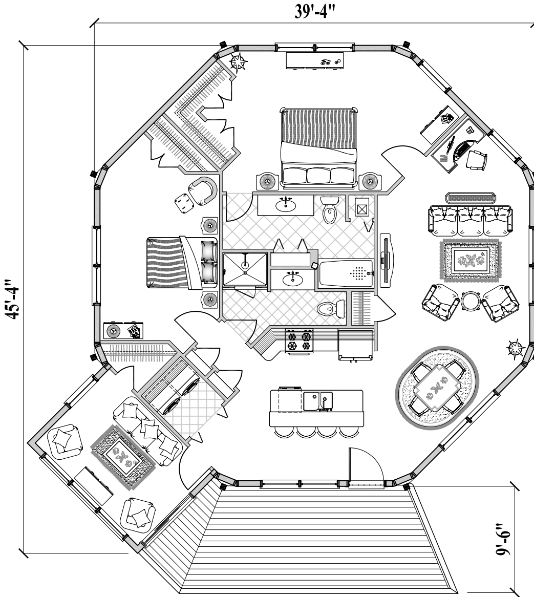
Floor Plan (Total 1,415 sq. ft. or 131.5 m 2 )
