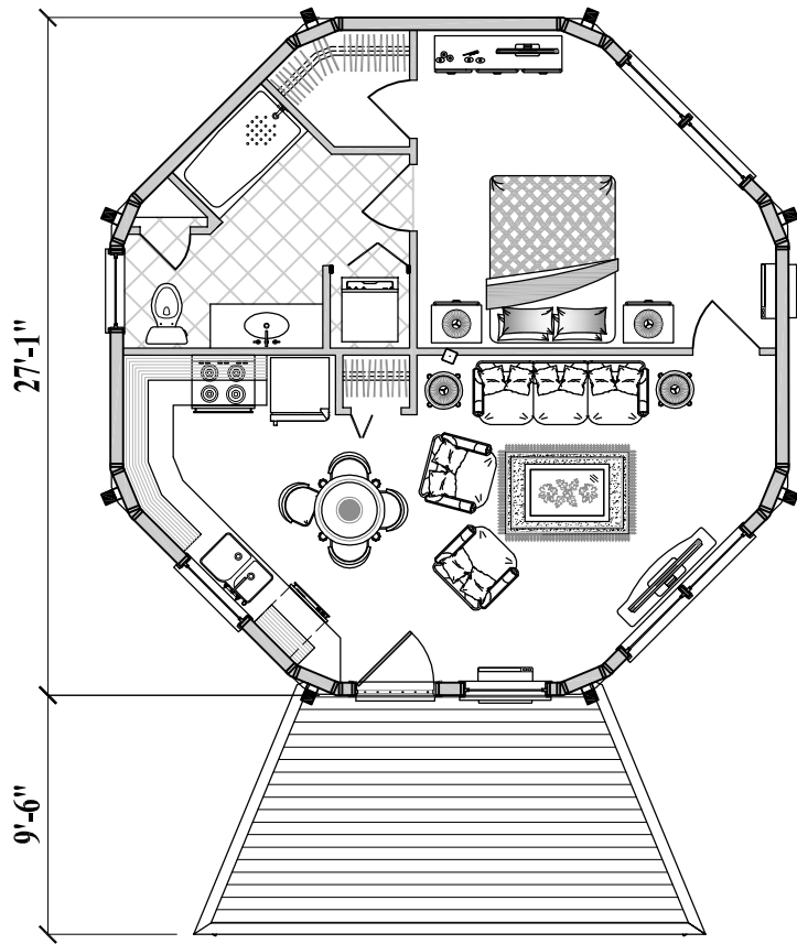
Floor Plan (Total 600 sq. ft. or 56 m 2 )
