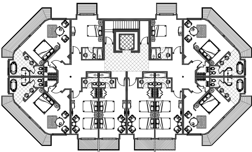
Level 4 Floor Plan
