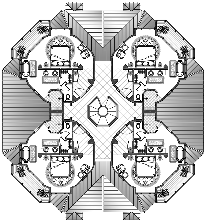
Floors 2 & 3 Plan
