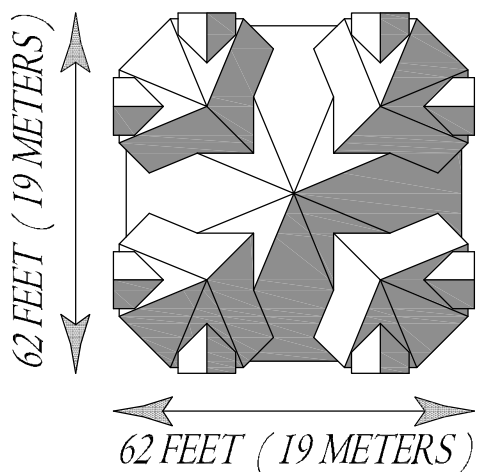
Floors 2 & 3 Plan
