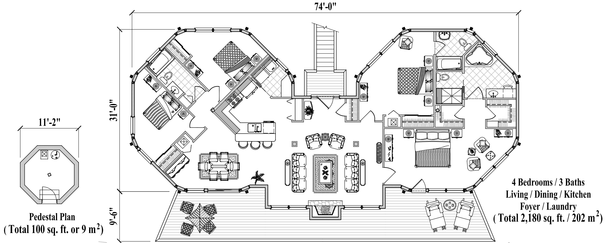
Floor Plan (1,980 sq. ft. or 184 m 2 )
