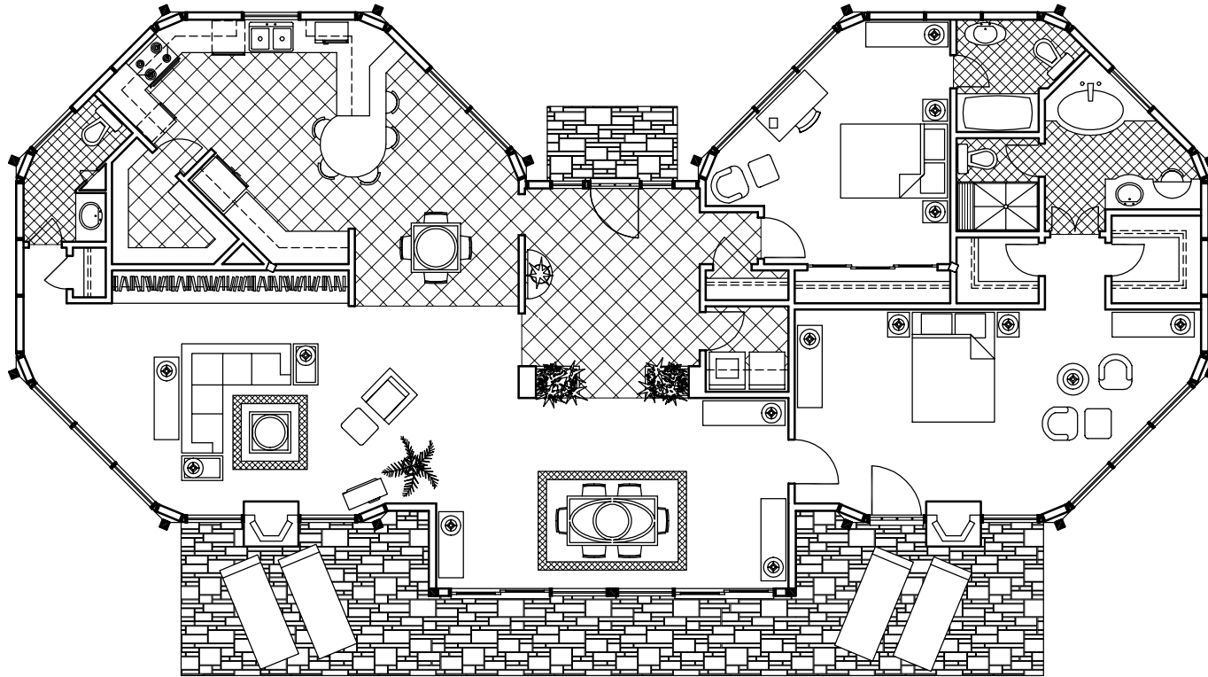
Floor Plan (1,980 sq. ft.)
