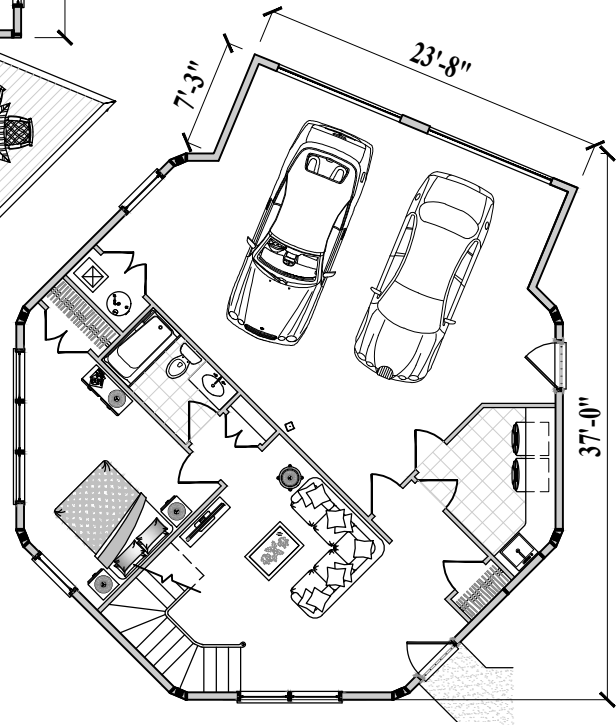
Lower Floor Plan (1250 sq. ft. or 116 m 2 )
