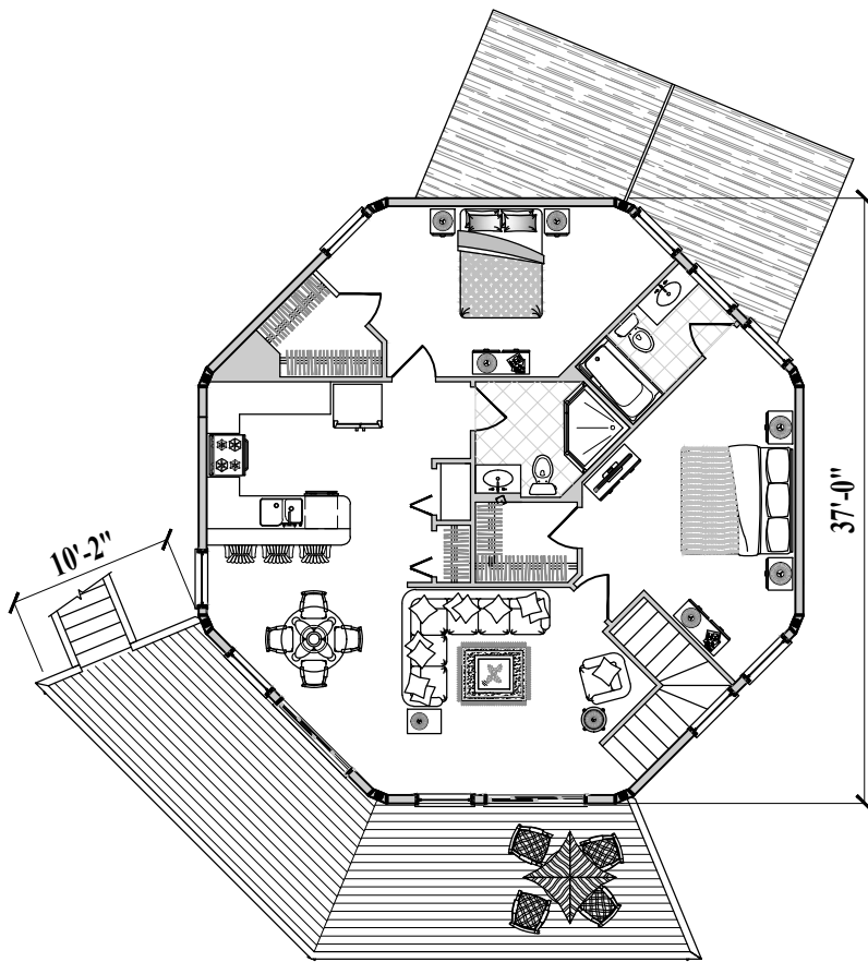
Upper Level Floor Plan (1,135 sq. ft. or 105m 2 )
