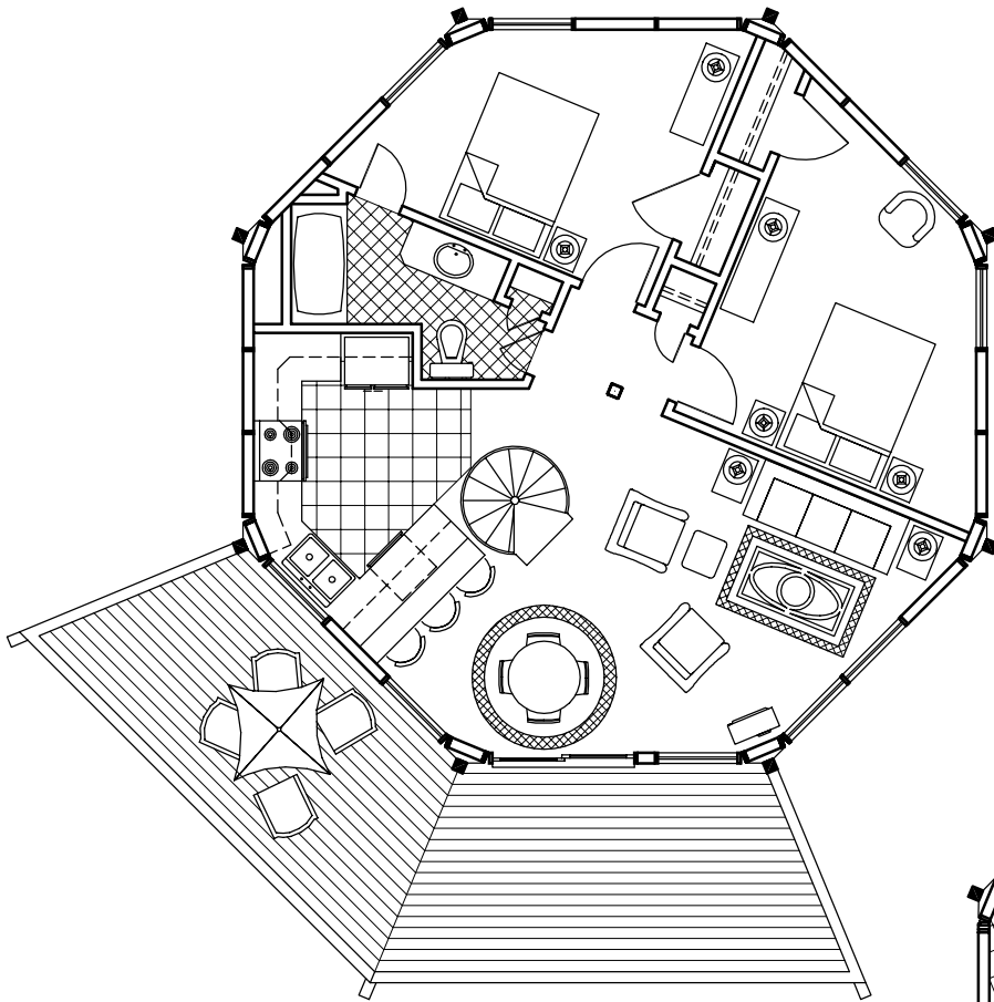
Upper Floor Plan (800 sq. ft.)
