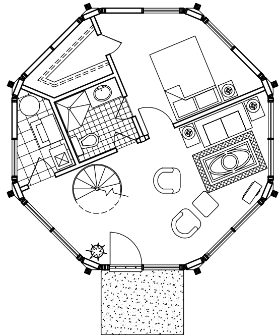
Lower Floor Plan (475 sq. ft.)
