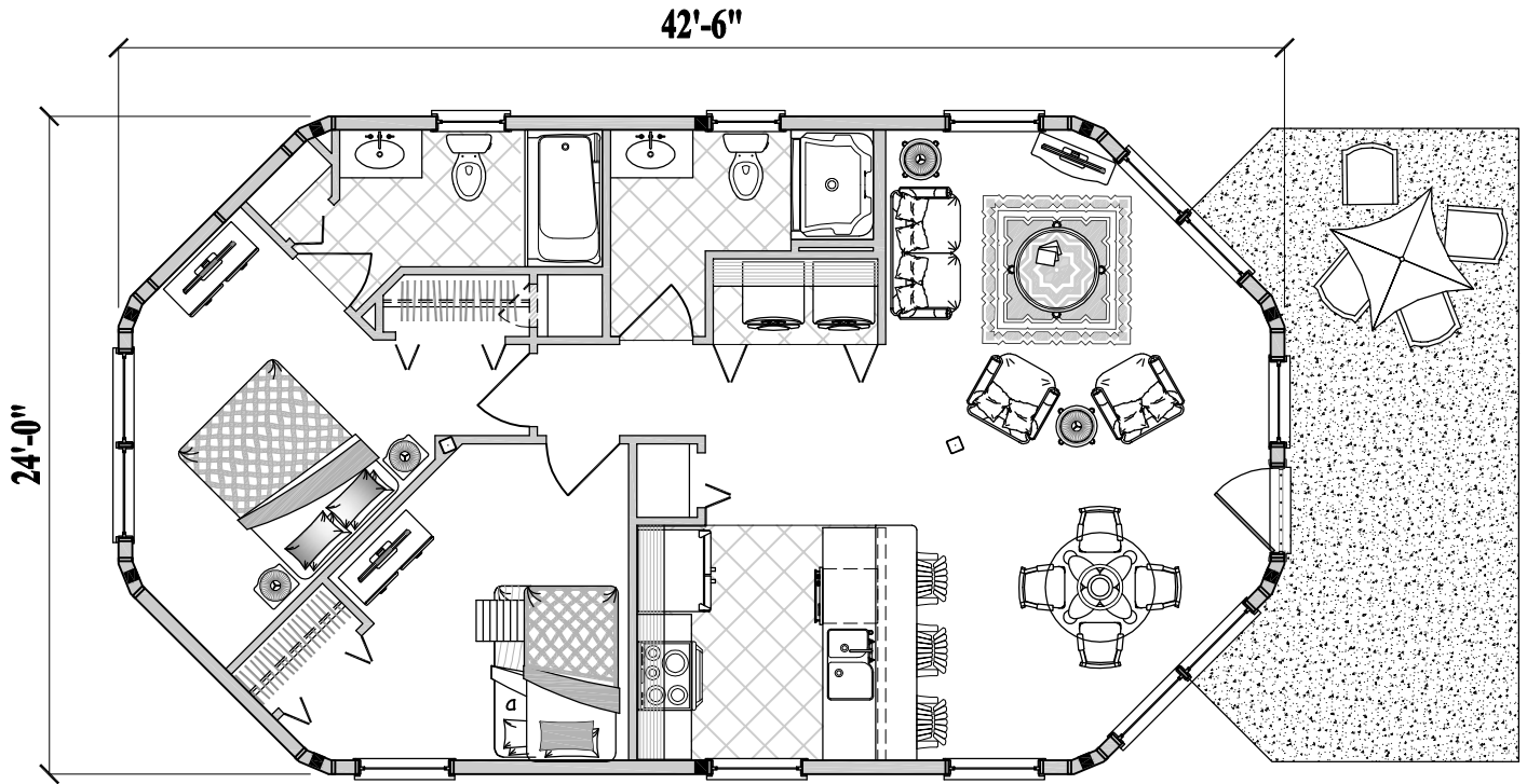
2 Bedroom / 2 Bath Living / Dining / Kitchen / Laundry (Total 920 sq. ft. or 85.5 m 2 )
