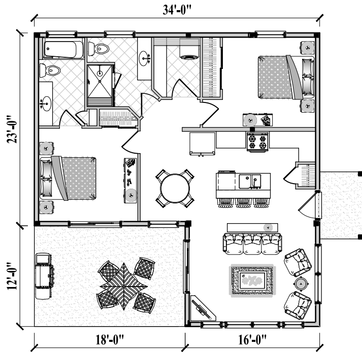
Floor Plan (975 sq. ft. or 90 m 2 )
