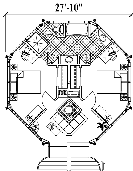
Upper Floor Plan (600sq. ft.)
