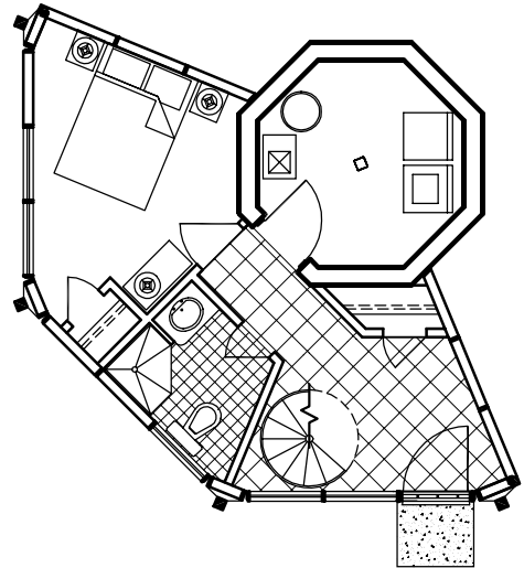
Lower Floor Plan (400 sq. ft.)
