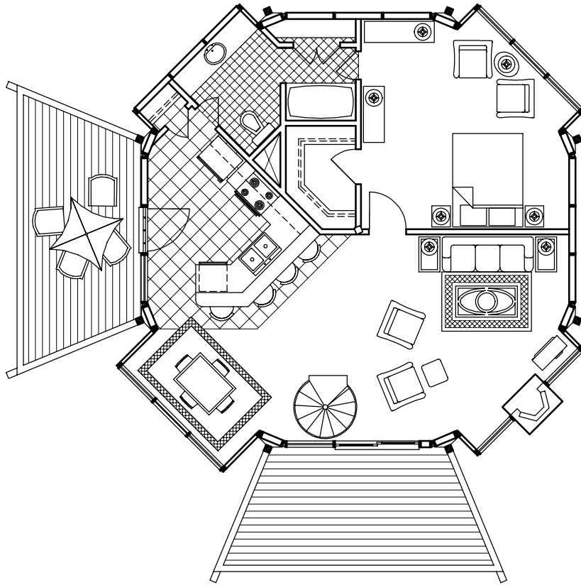
Upper Floor Plan (925 sq. ft.)
