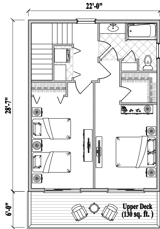
Upper Floor Plan (630 sq. ft. or 58.5 m 2 )
