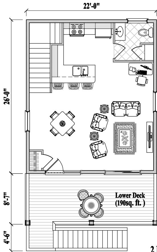
Lower Floor Plan (570 sq. ft. or 52.9 m 2 )
