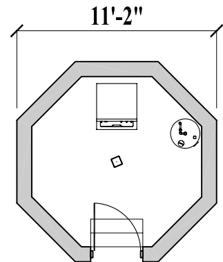
Pedestal Plan (Total 100 sq. ft. or 9 m 2 )
