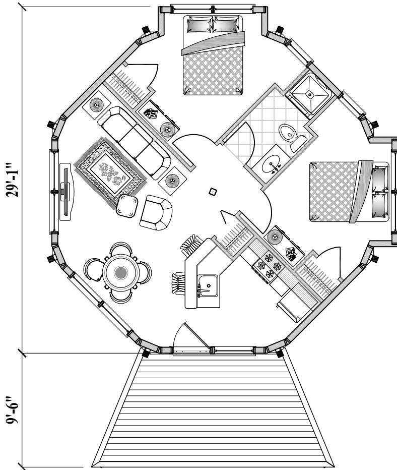
Floor Plan (Total 640 sq. ft. or 60 m 2 )
