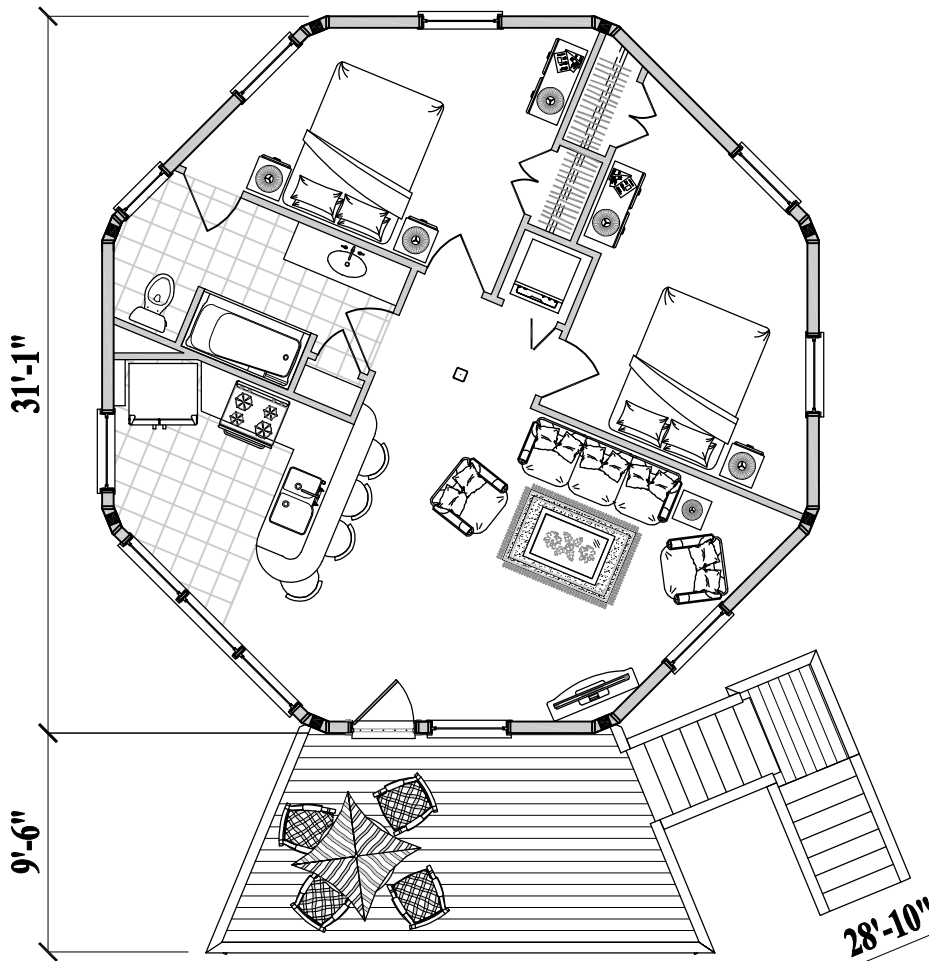
Upper Floor Plan ( 800 sq. ft. or 74.3 m 2 )
