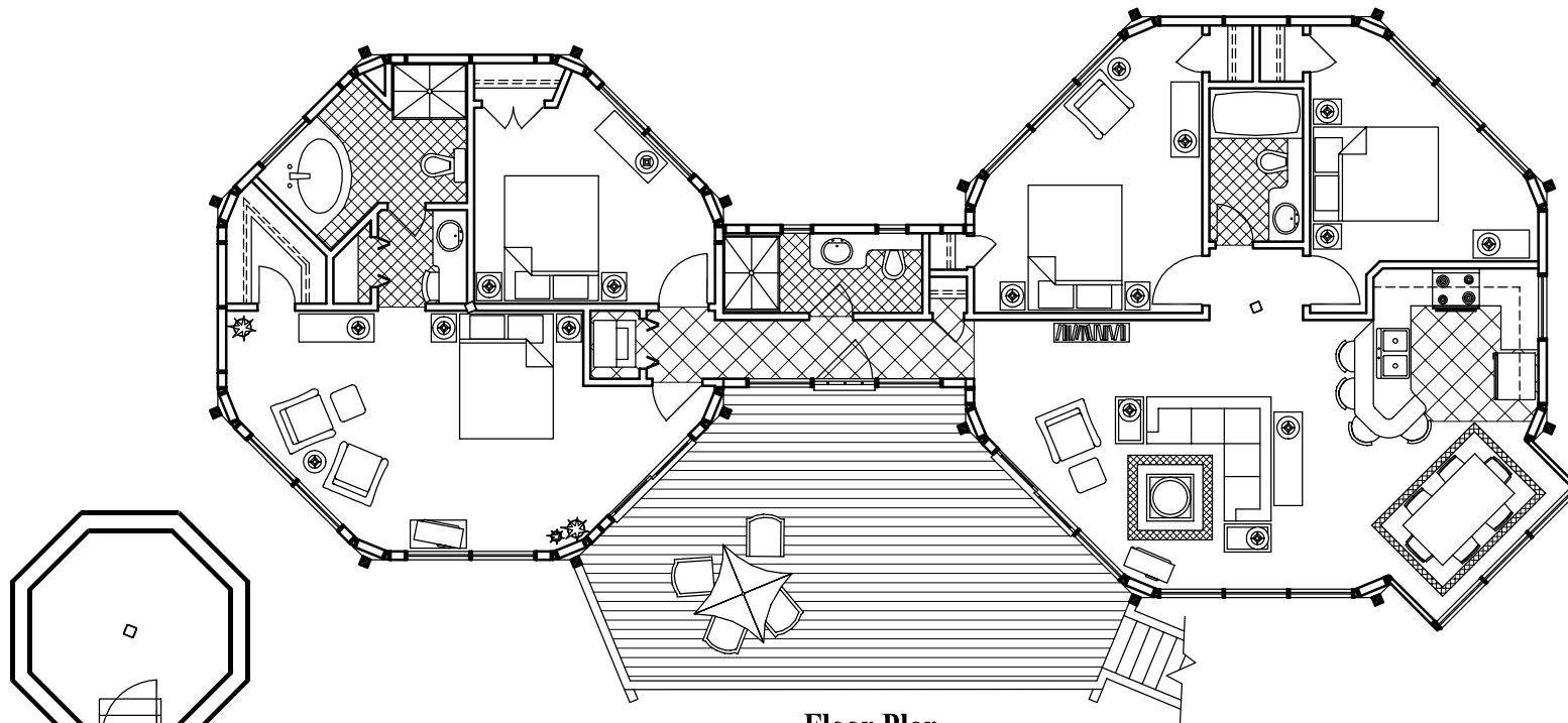
Floor Plan (1,600 sq. ft.)
