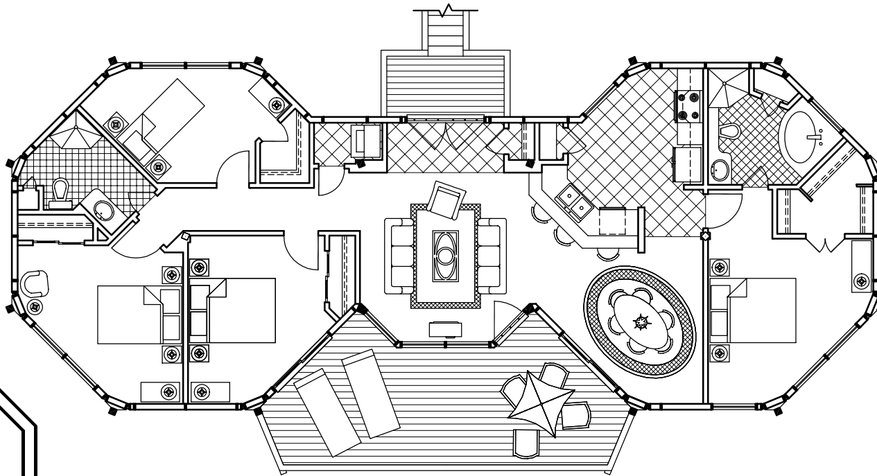
Floor Plan (1,450 sq. ft.)
