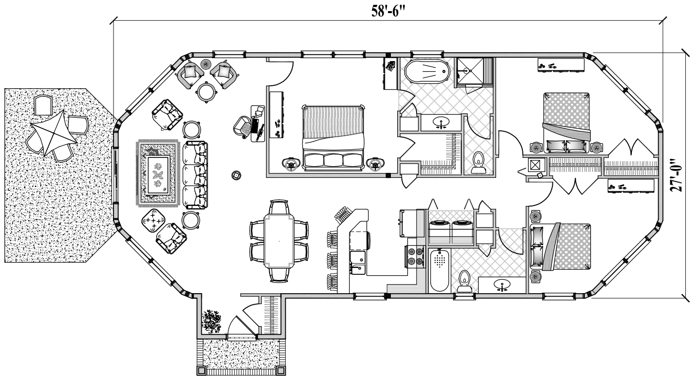
3 Bedroom / 2 Bath Living / Dining / Kitchen / Laundry ( Total 1,560 sq. ft. or 145 m 2 )
