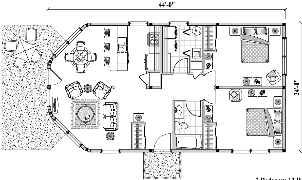
2 Bedroom / 1 Bath Living / Dining / Kitchen / Laundry ( Total 1,005 sq. ft. or 93 m 2 )
