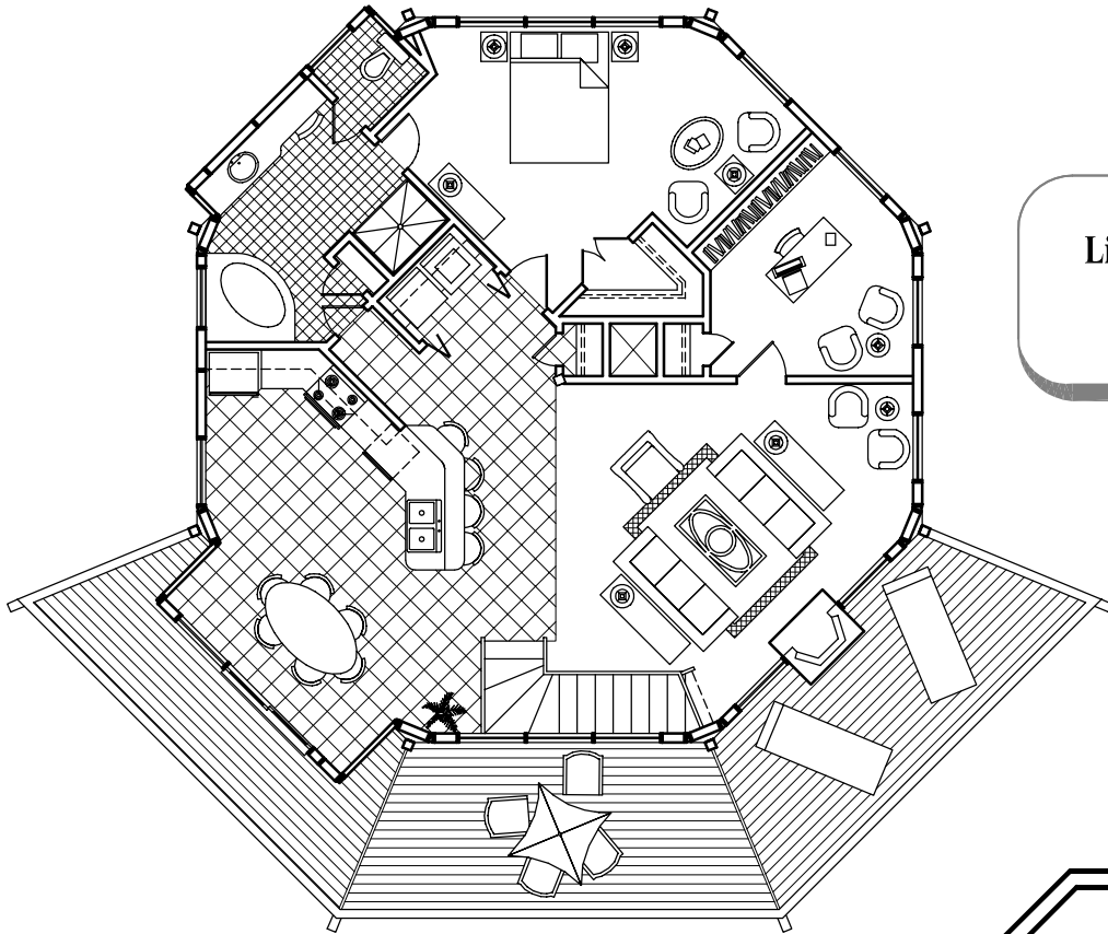
Upper Floor Plan (1,200 sq. ft.)
