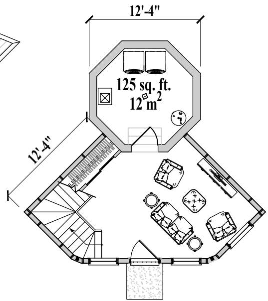
Lower Floor Plan (Total 390 sq. ft. or 35 m 2 including Pedestal)
