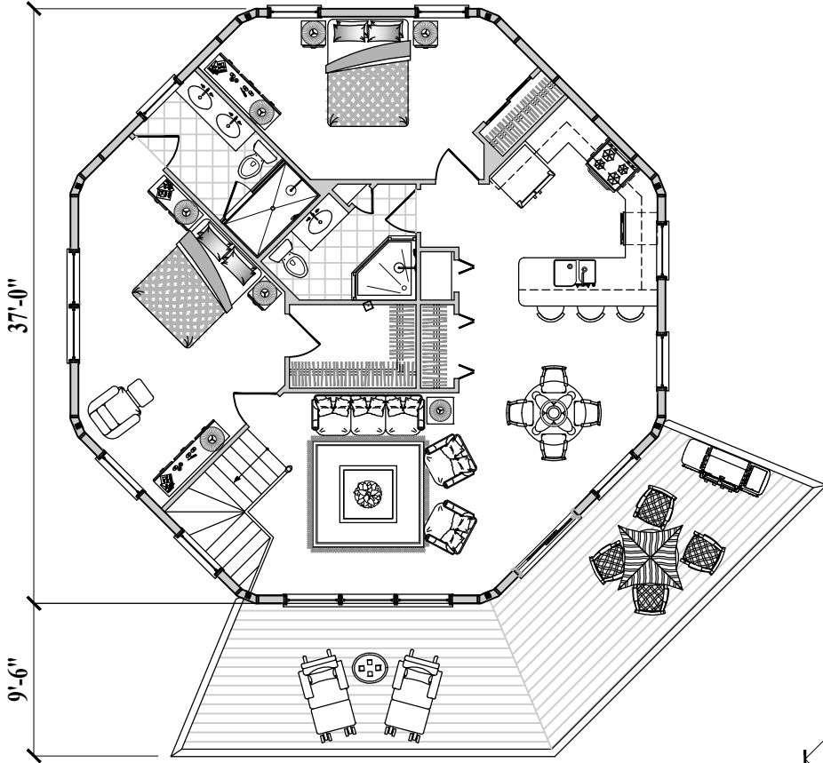
Floor Plan (Total 1,135 sq. ft. or 105 m 2 )
