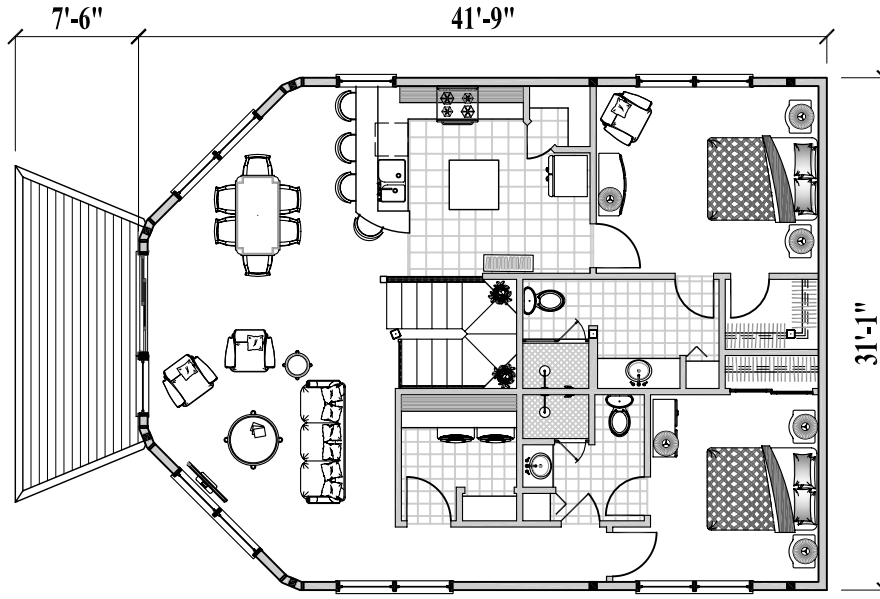
Upper Floor Plan ( 1,215 sq. ft. or 112.9 m 2 )
