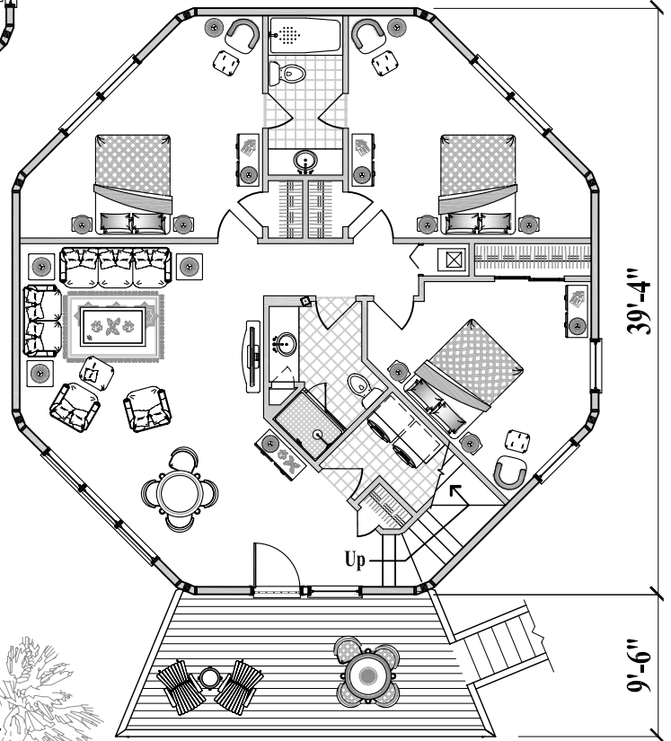
Lower Floor Plan (1,280 sq. ft. or 119 m 2 )
