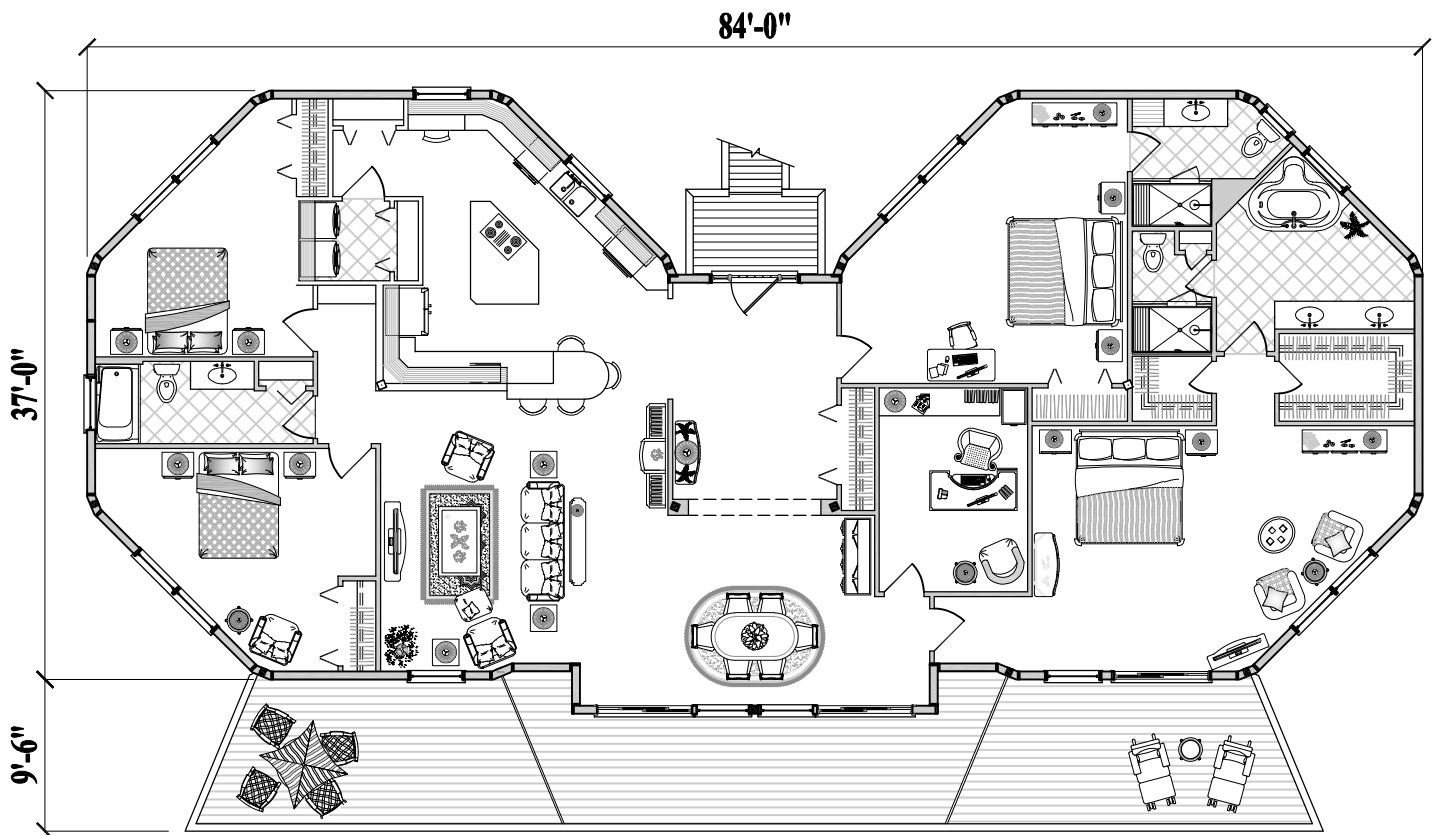
4 Bedrooms / 3 1/2 Baths Living / Dining / Kitchen / Office ( Total 2,685 sq. ft. or 249.5 m 2 )
