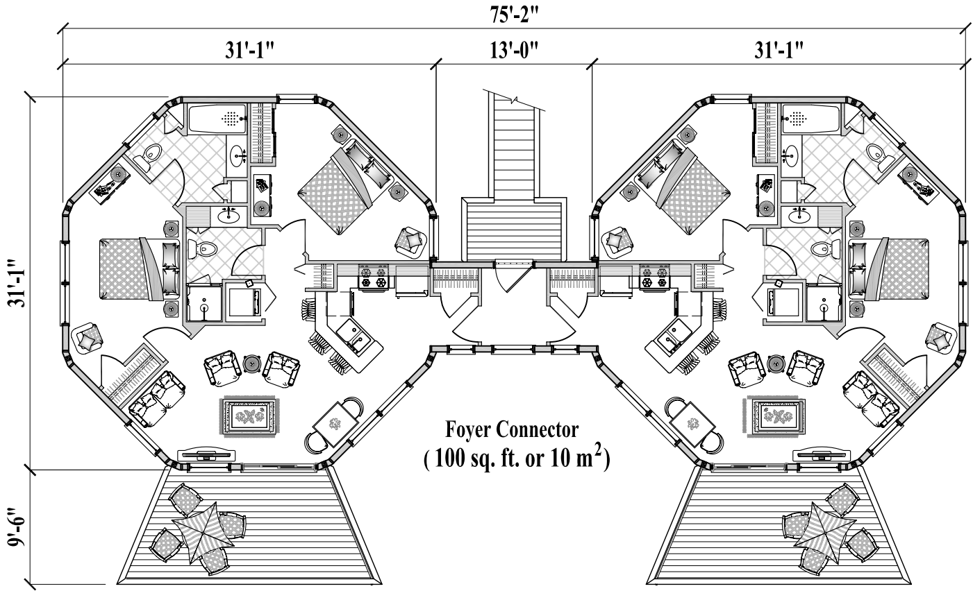
Floor plan ( 800 sq. ft. or 74 m 2 )
