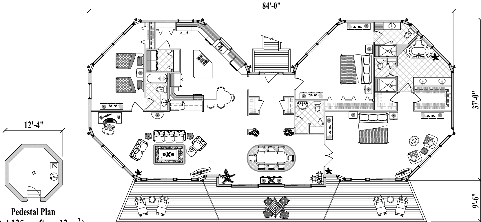
Floor Plan (2,665 sq. ft. or 247 m 2 )
